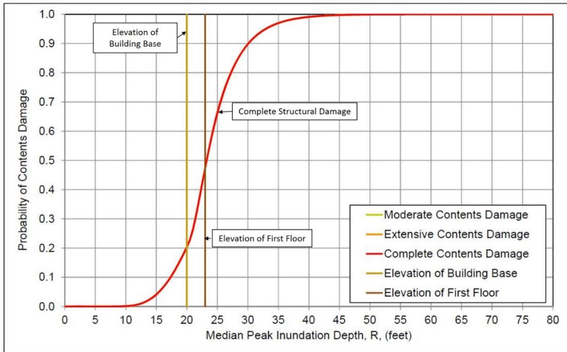
Figure 8-3 Example Fragility Curves for Contents Damage due to Tsunami Flood – Older One-Story Wood Buildings (W1 – PC)
