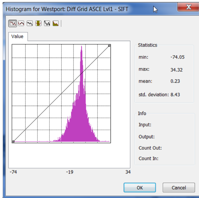
Figure 4-17 Difference Grid Histogram – Westport, WA
