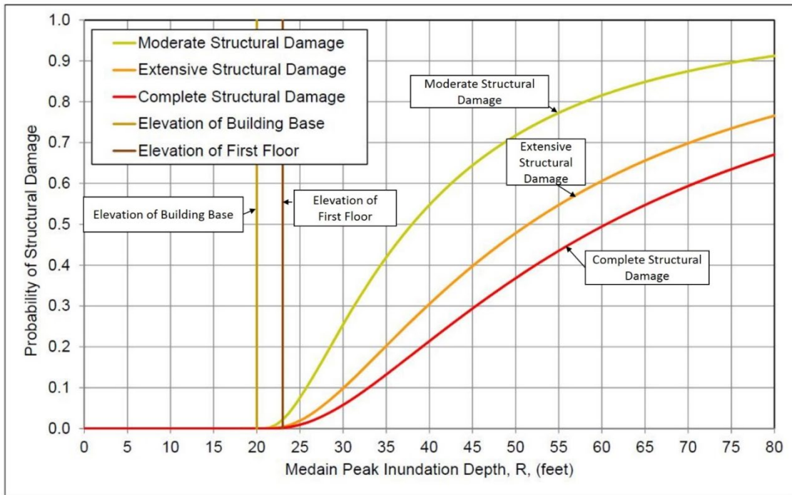
Figure 8-5 Example Fragility Curves for Structural System Damage Due to Tsunami Flow– Older Five-Story Concrete Buildings (C2M – PC)
