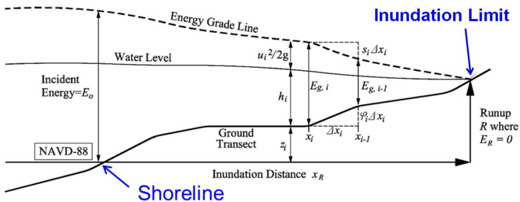
Figure 4-13 ASCE Energy Grade Line Analysis Approach
