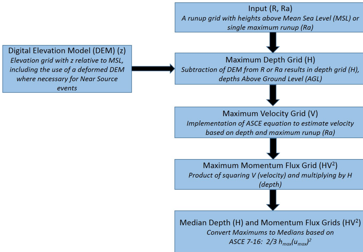
Figure 4-10 Flowchart for Level 1 (Basic) Methodology
