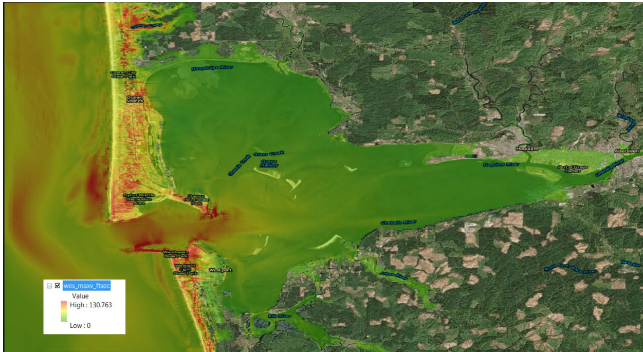
Figure 4-15 SIFT Model Velocity Grid for the Cascadia L1 Scenario, Westport, WA
