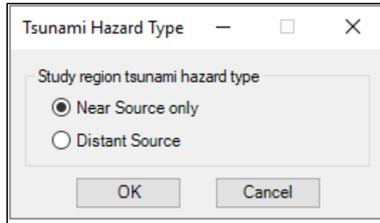
Figure 11-8 Tsunami Hazard Type
