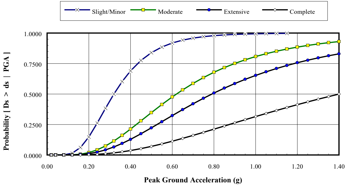
Figure 7-8 Fragility Curves at Various Damage States for Seismically Designed Railway Bridges Subject to Peak Ground Acceleration
