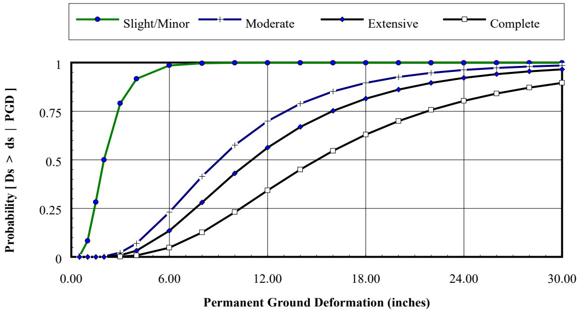
Figure 7-9 Fragility Curves at Various Damage States for Seismically Designed Railway Bridges Subject to Permanent Ground Deformation
